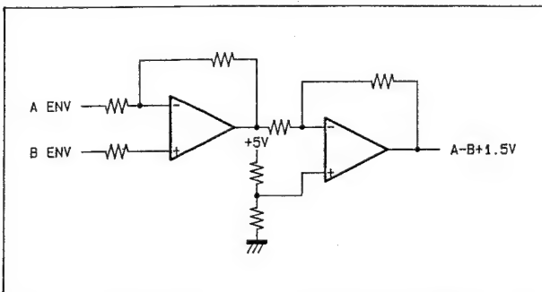
Fig. 4-4-13. RF Envelope Interface Circuit (CS-27 Board)
